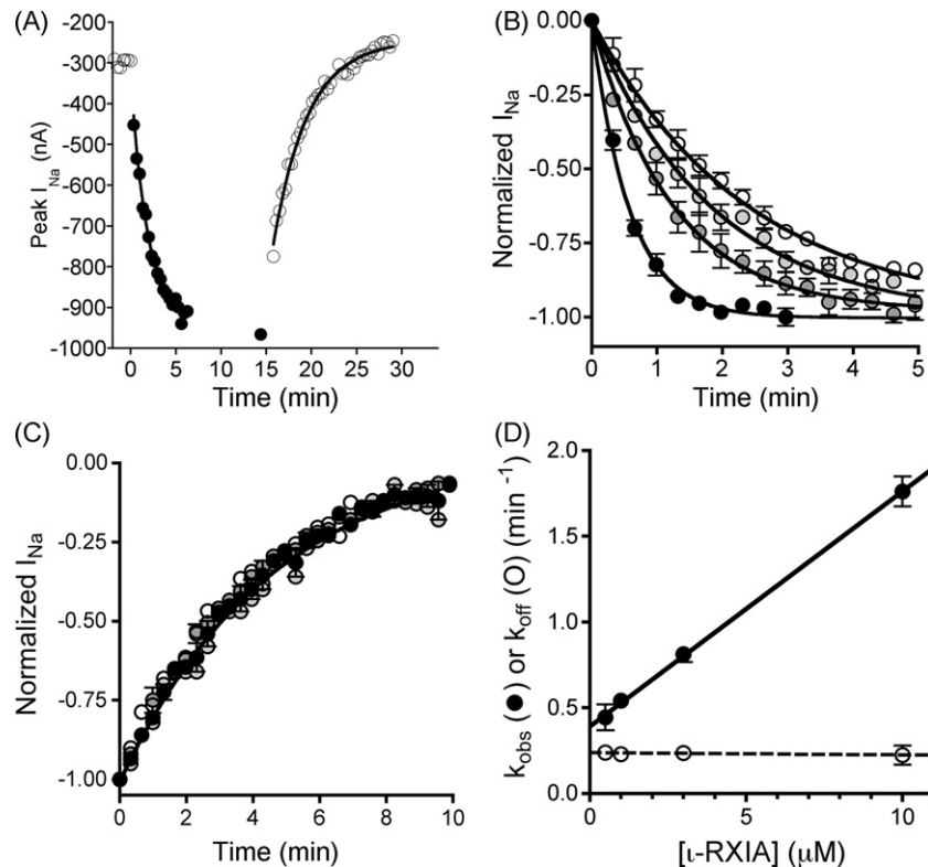
Fig. 4 – Kinetics of the modulation of \text{Na}_V1.6/\beta 1 by \iota -RXIA. Oocytes were used essentially as described in Fig. 2, and the peak I_{\text{Na}} in response to a V_{\text{step}} to -30 mV from a holding potential of -100 mV was measured at different times during the exposure to and washout of \iota -RXIA. (A) Representative time course of I_{\text{Na}} during exposure to 3 \mu\text{M} \iota -RXIA (closed circles) and its subsequent washout (open circles). Absence of points for 5 min in middle of plot reflects period when I - V data were being acquired. Single-exponential best-fits of the data provided k_{\text{obs}} (the observed rate constant for the toxin-induced increase in I_{\text{Na}} ) and k_{\text{off}} (the rate constant of recovery following washout). Values of k_{\text{obs}} and k_{\text{off}} for illustrated curves were 0.65 and 0.24 \text{min}^{-1} , respectively. (B) Time course of normalized peak I_{\text{Na}} upon exposure to 0.5, 1, 3, and 10 \mu\text{M} \iota -RXIA (from white to progressively darker circles, respectively). (C) Time course of normalized peak I_{\text{Na}} following washout of \iota -RXIA (symbols as in B). The data points largely overlap, and the best fit single-exponential curve for all of them is shown, yielding an aggregate k_{\text{off}} of 0.227 \pm 0.007 . (D) Plot of k_{\text{obs}} (closed circles) and k_{\text{off}} (open circles) versus [\iota\text{-RXIA}] , from data shown in (B) and (C), respectively. Values for k_{\text{obs}} increased linearly with peptide concentration, best-fit linear regression line (solid curve) has slope of 0.137 \pm 0.002 \mu\text{M}^{-1} \text{min}^{-1} and Y-intercept of 0.394 \pm 0.011 \text{min}^{-1} . In contrast, k_{\text{off}} values remained invariant, with average value of 0.229 \pm 0.021 \text{min}^{-1} . Each data point represents mean \pm S.E. ( N = 3 oocytes).
