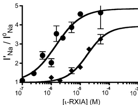
Fig. 5 – Modulation \text{Na}_v1.6/\beta1 and 1.2/\beta1 as a function of \iota -RXIA concentration at steady-state. Current measurements in response to a V_{\text{step}} to -30 \text{ mV} were made as in Fig. 4, and modulation is expressed as a ratio of peak currents, I'_{\text{Na}}/I^0_{\text{Na}} , where I'_{\text{Na}} and I^0_{\text{Na}} were obtained in toxin and control solution, respectively. Effect of \iota -RXIA on \text{Na}_v1.6/\beta1 (circles) and \text{Na}_v1.2/\beta1 (diamonds) measured at steady-state, solid line represents data fit to the equation, Y = (\text{Top} - 1)/(1 + 10^{(\text{Log EC}_{50} - \text{Log}[\iota\text{-RXIA}]) \times n_H}) , where n_H is the Hill coefficient. Respective \text{EC}_{50} values for \text{Na}_v1.6/\beta1 and 1.2/\beta1 were 1.80 \mu\text{M} (95% CI: 0.93\text{--}3.60 \mu\text{M} ) and 17.78 \mu\text{M} (95% CI: 4.70\text{--}67.21 \mu\text{M} ) and n_H values were 1.04 \pm 0.26 and 1.24 \pm 0.44 . Each point represents mean \pm S.E. ( N = 3 oocytes).
