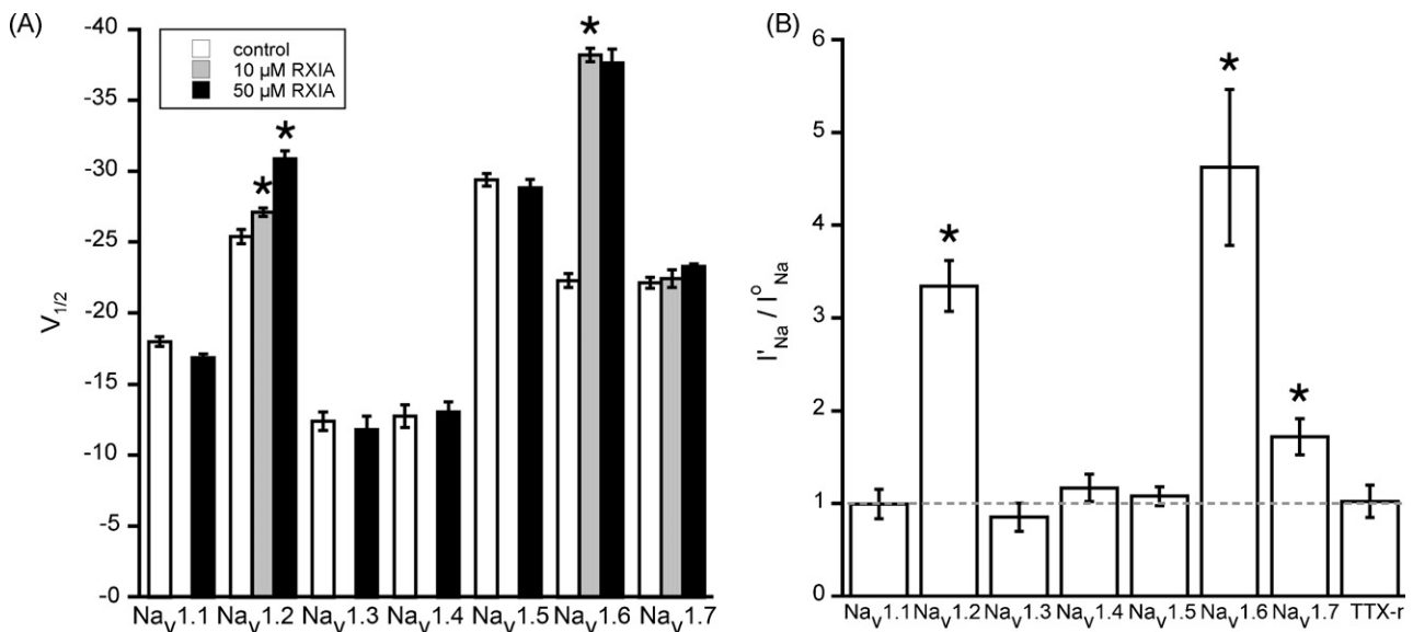
Fig. 3 – Effect of \iota -RXIA on Na_v1.1 through Na_v1.7 coexpressed with \beta1 in Xenopus oocytes and TTX-resistant Na channels in dissociated neurons from mouse DRG. Oocytes were used as in Fig. 2, and neurons were whole-cell clamped and TTX-resistant I_{Na} were recorded as described in Section 2. (A) V_{1/2} of the voltage-dependence of activation in controls (white bars) and in the presence of 10 \mu\text{M} (gray bars) or 50 \mu\text{M} (black bars) \iota -RXIA. In 10 \mu\text{M} \iota -RXIA, V_{1/2} 's of only Na_v1.2/\beta1 and 1.6/\beta1 differed significantly from control. In 50 \mu\text{M} \iota -RXIA, V_{1/2} of Na_v1.6/\beta1 remained unchanged, that of Na_v1.2/\beta1 changed further, and those of Na_v1.1/\beta1 , 1.3/\beta1 , 1.4/\beta1 , 1.5/\beta1 , and 1.7/\beta1 remained insignificantly different from controls. (B) Ratio of I'_{Na}/I^0_{Na} for V_{step} to -30 mV, where I'_{Na} and I^0_{Na} are peak I_{Na} in 50 \mu\text{M} \iota -RXIA and control, respectively. The ratio measurement shows that in addition to Na_v1.2/\beta1 and 1.6/\beta1 , Na_v1.7/\beta1 was also significantly up-modulated by 50 \mu\text{M} \iota -RXIA. I'_{Na}/I^0_{Na} value of none of the other Na channels differed significantly from 1, indicating they were not affected even at this high toxin concentration. Bars represent mean \pm SE ( N = 3 ). * p < .05 , compared to bar immediately to its left (A) or compared to value of 1 (B).
