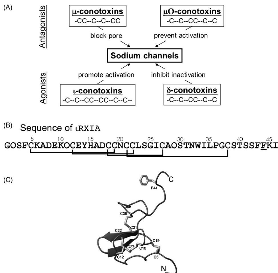
Fig. 1 – (A) Four families of peptide conotoxins that target Na channels. Members in the upper two, \mu - and \mu O-conotoxins, inhibit Na channels, whereas those in the lower two, \iota - and \delta -conotoxins, are agonist. The cysteine framework of each peptide family is illustrated. All cysteines are disulfide-bonded, rendering each peptide into a compact structure. (B) The sequence of \iota -RXIA, the iota-conotoxin studied in this report, where O is hydroxyproline, and the underlined F (residue 44) is the D-enantiomer of phenylalanine. The synthetic homologue, \iota -RXIA[L-Phe44], is identical to \iota -RXIA except residue 44 is an L-phenylalanine. The disulfide bridges between Cys residues are indicated. (C) Ribbon structure of \iota -RXIA determined by NMR spectroscopy [20]. Locations of the Cys residues and their disulfide linkages are indicated; also shown is the side chain of D-Phe44. This figure was prepared using PyMol ( http://www.pymol.org ).
