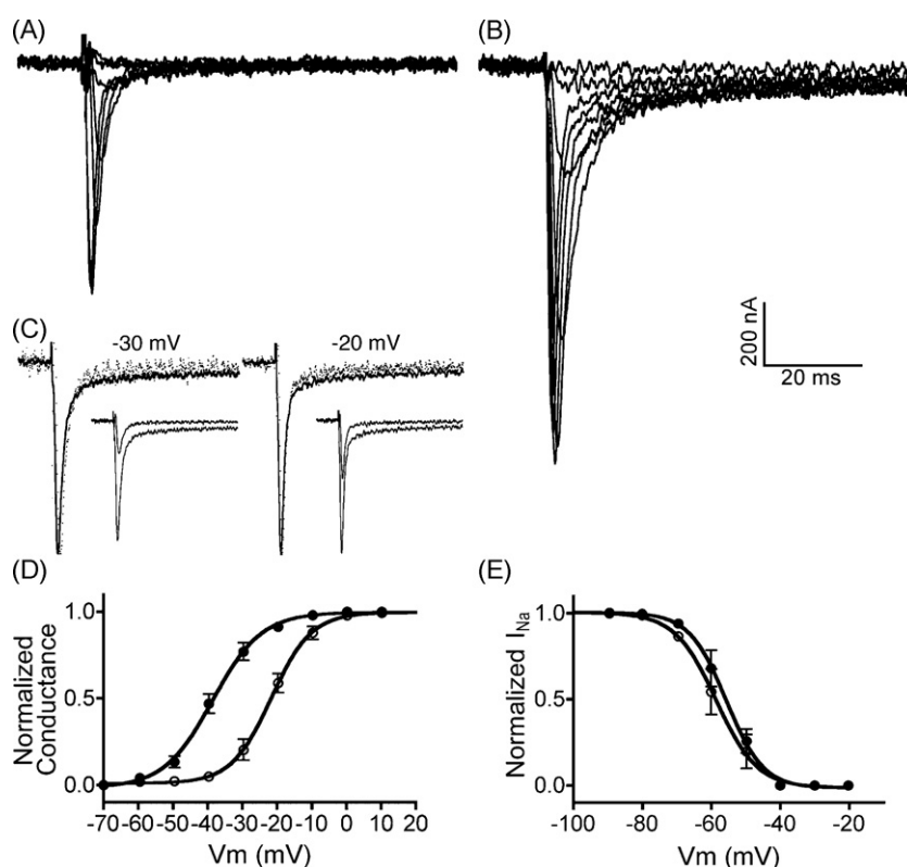
Fig. 2 – \iota -RXIA modulates the activity of Na_v1.6 coexpressed with \beta 1 in Xenopus oocytes by shifting its voltage-dependence of activation. Oocytes were two-electrode clamped at a holding potential of -100 mV, and V_m was stepped in 10 mV increments as described in Section 2. Representative current records for voltage steps ranging from -60 to 10 mV in the absence (A) and presence (B) of 10 \mu M \iota -RXIA. (C) Normalized current traces from A and B in response to the voltage step to -30 mV (left) and -20 mV (right), in the absence (dots) and presence (solid line) of 10 \mu M \iota -RXIA; each pair of responses to a given voltage step largely overlap. Insets show corresponding traces non-normalized. Voltage sensitivity of activation (D) and inactivation (E) obtained in the absence (open circles) and presence (closed circles) of \iota -RXIA. The solid lines are best-fit curves to the Boltzmann equation. V_{1/2} values for activation in D were -22.38 \pm 0.48 (control) and -38.29 \pm 0.47 mV ( 10 \mu M \iota -RXIA) with respective slope factors of -6.08 \pm 0.42 and -7.53 \pm 0.41 mV. V_{1/2} values for inactivation in (E) were -58.71 \pm 1.03 (control) and -55.73 \pm 0.75 mV ( 5 \mu M \iota -RXIA) with respective slope factors of 5.98 \pm 0.90 and 5.37 \pm 0.61 mV. Each data point represents mean \pm SE ( N = 3 oocytes).
