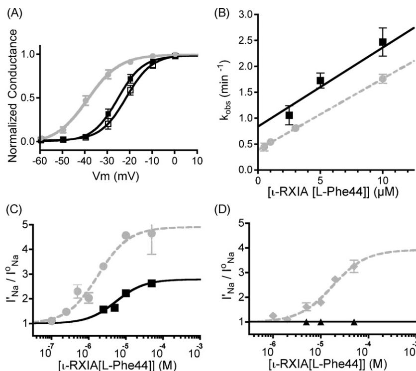
Fig. 6 – Comparison of the modulation of \text{NaV1.6}/\beta 1 and \text{NaV1.2}/\beta 1 by \iota -RXIA[L-Phe44] and \iota -RXIA. Oocytes were tested essentially as described in Figs. 2–4. (A) Voltage dependence of activation of \text{NaV1.6}/\beta 1 in the absence (open squares) and presence of 50 \mu\text{M} \iota -RXIA[L-Phe44] (closed squares); respective V_{1/2} was -21.66 \pm 0.61 and -25.30 \pm 0.27 mV and slope factor was 5.75 \pm 0.54 and 5.58 \pm 0.23 mV. For comparison, the curve for \iota -RXIA from Fig. 2D is shown in gray. (B) Plot of k_{obs} vs. concentration of \iota -RXIA[L-Phe44] for \text{NaV1.6}/\beta 1 (black squares). Slope (or k_{on} ) was 0.152 \pm 0.008 \mu\text{M}^{-1} \text{min}^{-1} , and Y intercept (or extrapolated k_{off} ) was 0.841 \pm 0.145 \text{min}^{-1} , yielding a K_d of 5.52 \mu\text{M} . For comparison, the curve for \iota -RXIA (from Fig. 4D) is shown in gray. (C) Modulation of \text{NaV1.6}/\beta 1 as a function of \iota -RXIA[L-Phe44] concentration (black squares). EC_{50} was 5.45 \mu\text{M} (95% CI: 2.03 – 14.63 \mu\text{M} ) and n_H was 1.13 \pm 0.39 . For comparison, the curve for \iota -RXIA (from Fig. 5) is shown in gray; note that at or near saturating [peptide] its efficacy is about twice that of \iota -RXIA[L-Phe44]. (D) Modulation of \text{NaV1.2}/\beta 1 as a function of \iota -RXIA[L-Phe44] concentration (black triangles) yields a flat line, showing that the peptide had no effect on \text{NaV1.2}/\beta 1 . For comparison, the curve for \iota -RXIA (from Fig. 5) is shown in gray.
