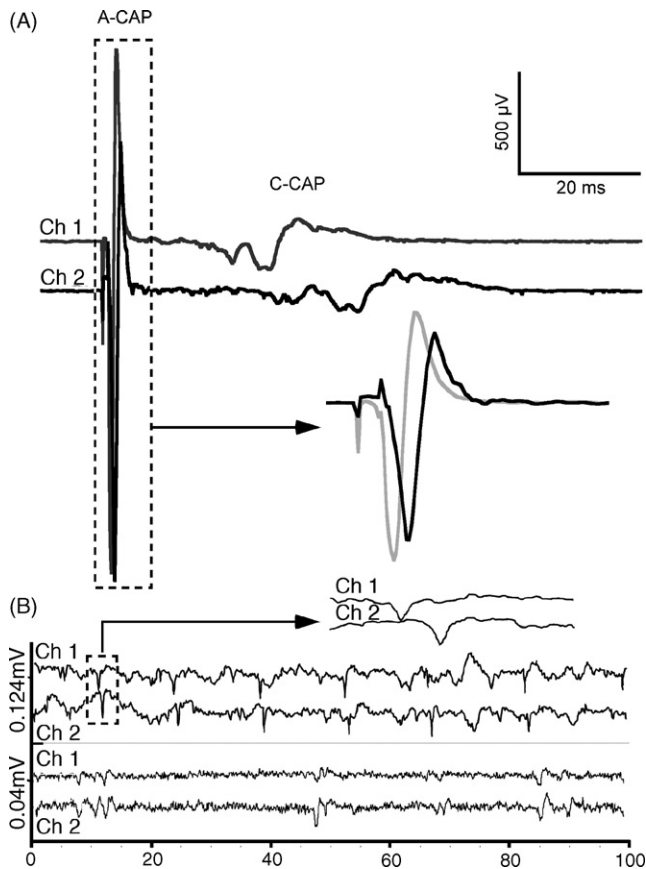
Fig. 7 – \iota -RXIA induces action potentials in A- and C-fibers in mouse sciatic nerve. Extracellular action potentials were recorded simultaneously from two locations along the nerve as described in Section 2, 7 mm apart. In each pair of traces, the upper (Channel 1) and lower (Channel 2) traces were recorded from a proximal versus distal location, respectively, relative to the site of electrical stimulus (A) or toxin-application (B). (A) Stimulus-evoked compound action potentials (CAPs) in control solution showing fast A-CAP with conduction velocity of 11.8 m/s, and slower C-CAP with conduction velocity in the range of 0.72–0.48 m/s. Region of A-CAPs enclosed by (10 ms wide) dashed box is shown in inset with baselines superimposed and reveals a \sim 0.6 ms temporal offset; note 1 ms stimulus artifact near start of traces. (B) “Spontaneous” action potentials induced by exposure to 0.05 \mu\text{M} \iota -RXIA; representative recordings of single-units with conduction velocities of about 10 (top pair) and 0.7 (bottom pair) m/s. Region of top pair of traces enclosed by (5 ms wide) dashed box is shown in inset, revealing a \sim 0.7 ms temporal offset of this unit corresponding to that of an A-fiber. Lower trace in bottom pair of traces has been shifted leftward by 9.5 ms and reveals near coincidence of units corresponding to those of C-fibers.
